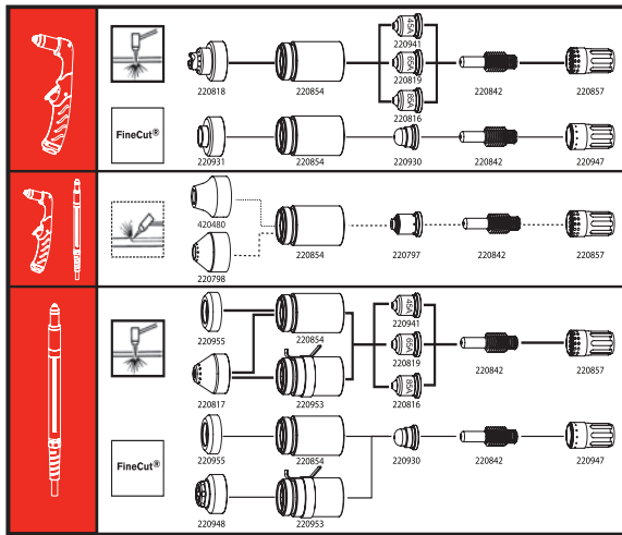
Consumable label
